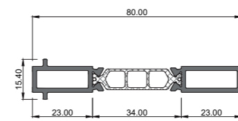
COR-3798 Versatile union of frames
